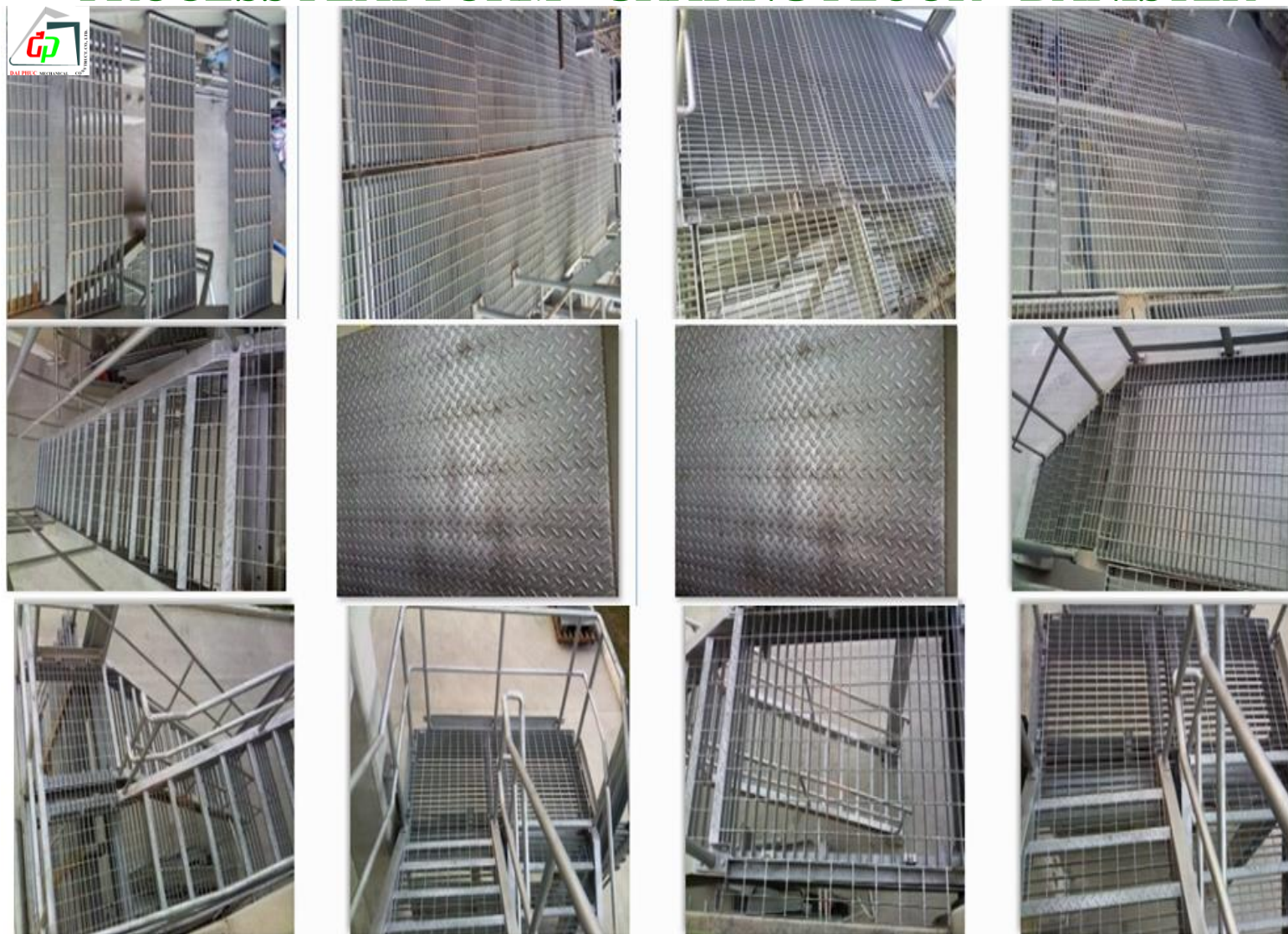
PROCESS PLAT FORM - GRATING FLOOR - BANISTER
